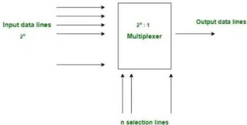
Fig3.1: Multiplexer
